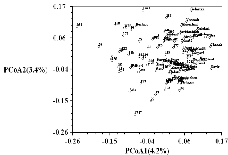
Fig. 4. Principle coordinate analysis plot of 101 bread wheat cultivars and breeding lines revealed by ISSR data
