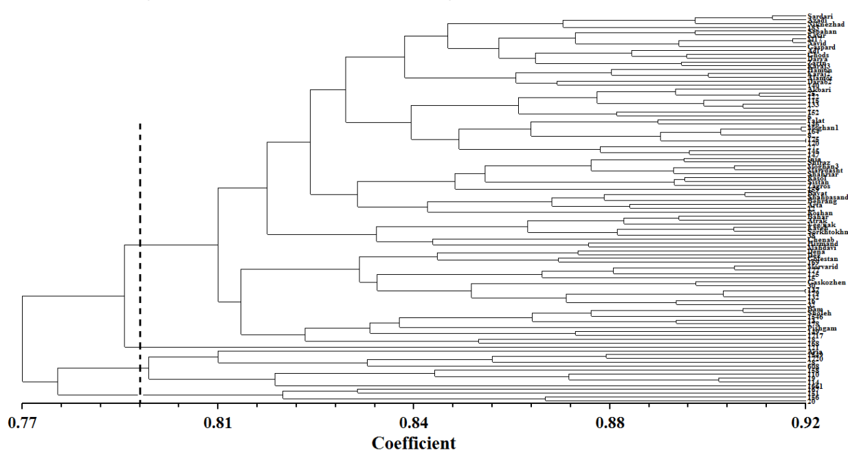
Fig. 3. Dendrogram of 101 bread wheat genotypes constructed with complete linkage method using Dice similarity coefficient based on 267 ISSR loci
